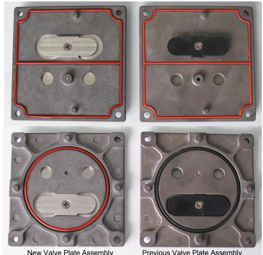
New Valve Plate Assembly
